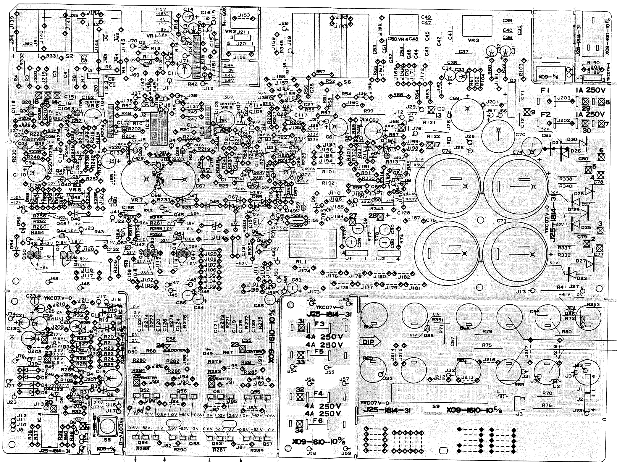
AUDIO AMP (X09-160*-.**) Component Side View
